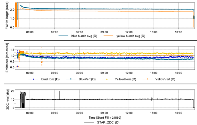
Figure 3: Bunch length, emittance, and ZDC collision rates at steady levels over 20-hour stores.
