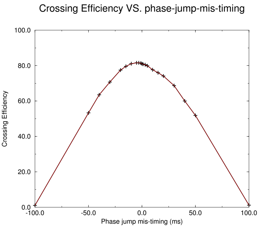
Figure 1: Crossing efficiency at different RF jump mis-timing.
