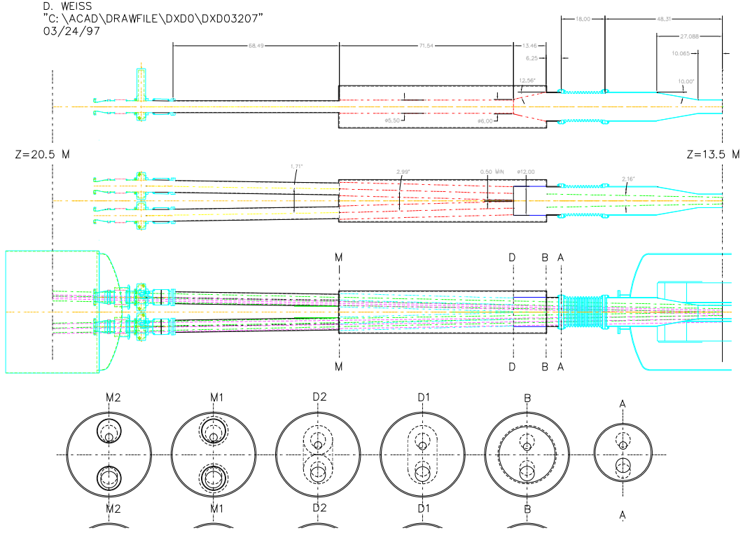
Figure 1: DX-D0 Interconnect
