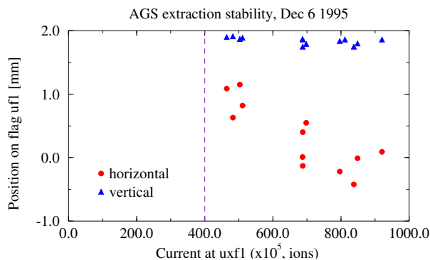
Figure 4: Stability of AGS extraction: position measured on flag UF1 at the beginning of the ATR versus intensity.
