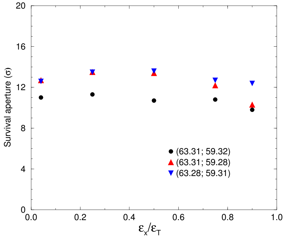
Figure 1: The survival aperture versus a direction in transverse plane. The data averaged over 10 seeds are shown for three different working points. 0.0 corresponds to the vertical direction while 1.0 is horizontal.
